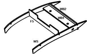
Step 1.2 and 3.2--detail of attachment of Wing Boss to Wing Saddles, other parts omitted.
